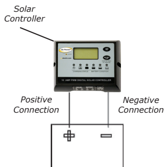
Single 12 Volt Battery 12 Volt Configuration Figure 3
