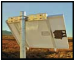
Series 4001 (Special Order) with SolarMount® standard rails for 2.5" (65 mm) Schedule 40 or 80 steel pole, outside dia. 2.875" (73.0 mm)
