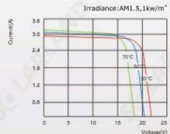
SLP050-12 I-V Curves
