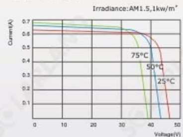
SLP020-24 I-V Curves
