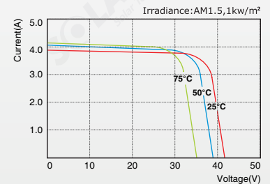
SLP120-24U I-V Curves
